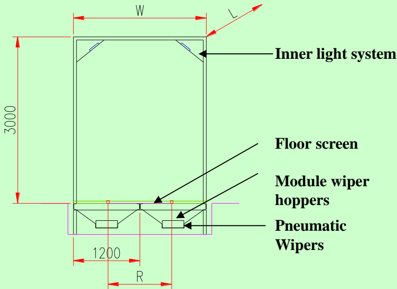
Cabinet section
