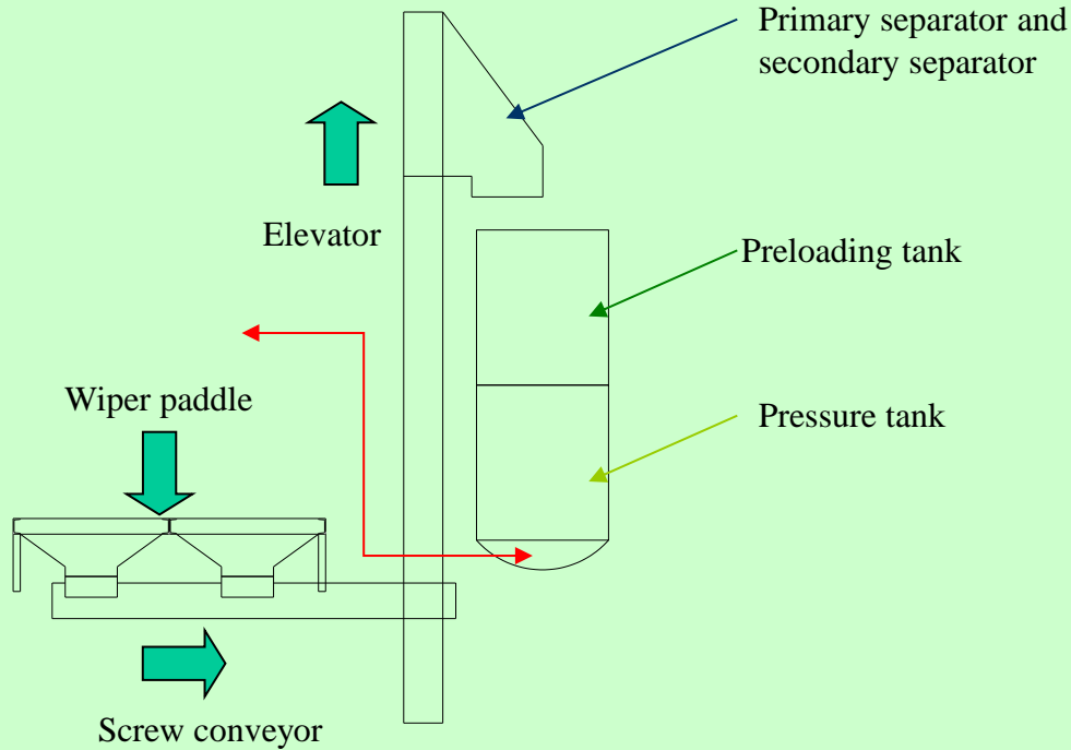
Schema of recycling system
